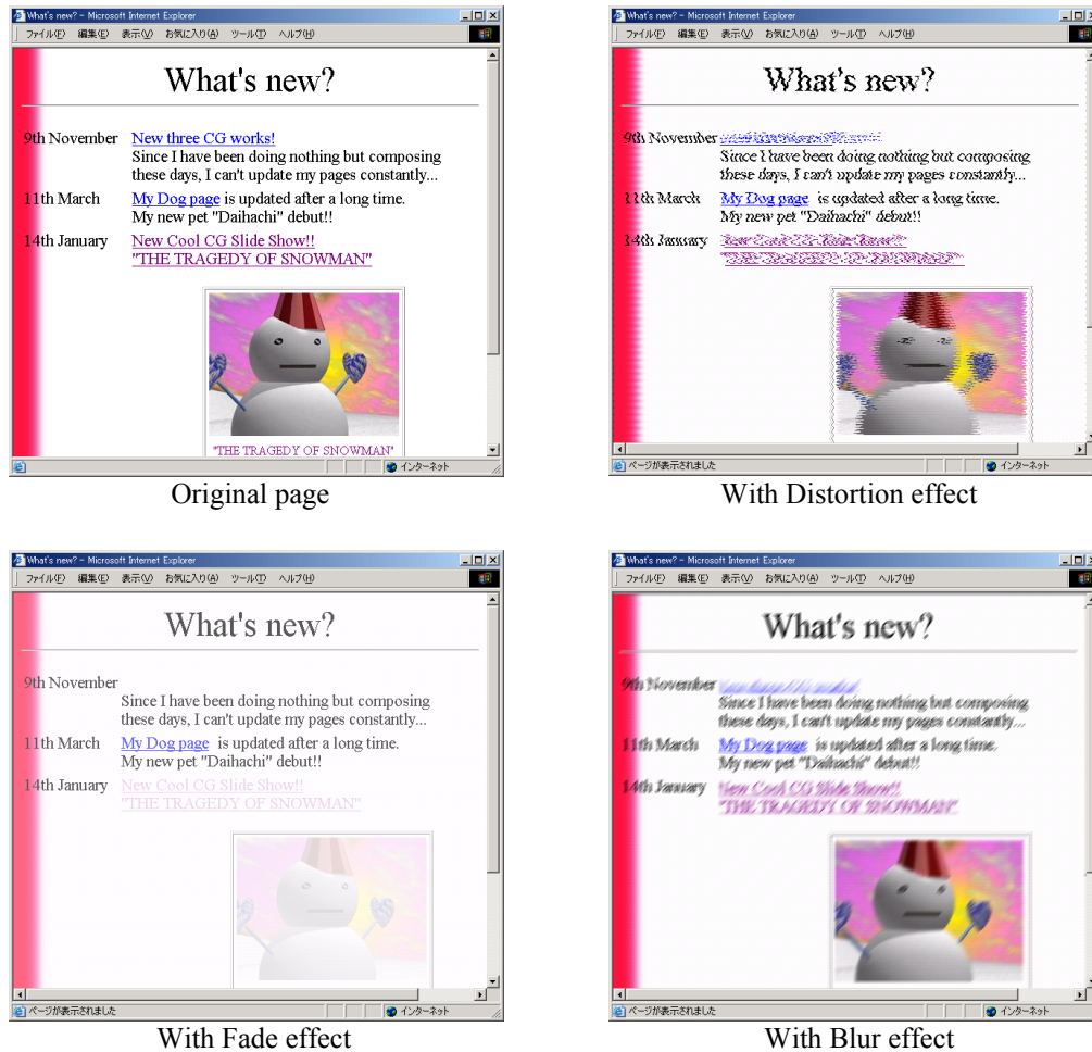
Figure 3: Examples of Distortion, Fade, and Blur effects.
